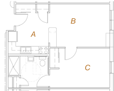
UNIT PLAN
